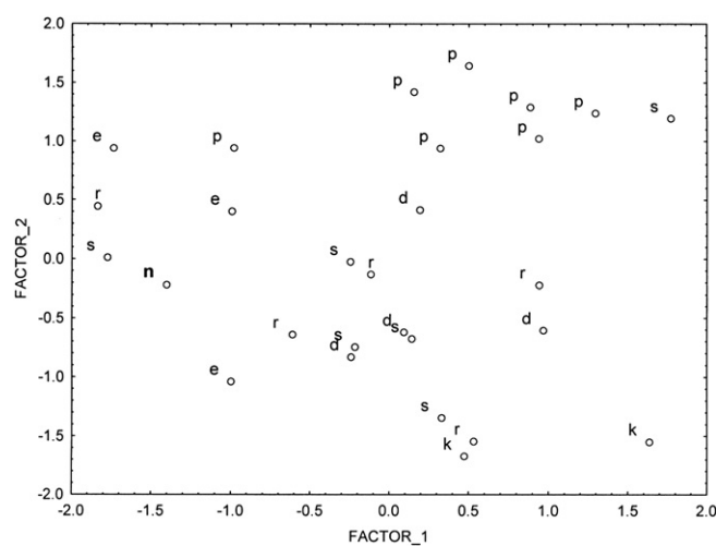
Fig. 7. Plot of factor scores of Factor 1 and Factor 2 from principal component analysis of bear mandibles. d – Ursus deningeri deningeri , Mosbach, Germany; e – U. etruscus ; k – U. deningeri kudarensis , Kudaro 1 Cave (layers 3–4), Georgia; n – Cherskiy; p – U. arctos pruinusos , Tibet, China, recent; r – U. savini rossicus , Siberia, Russia; s – U. savini savini , Bacton Forest Bed, Britain.
