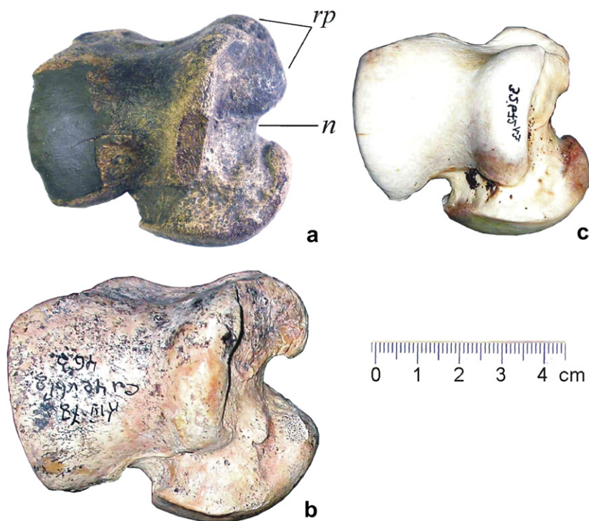
Fig. 8. Right astragali of cave bears (a, b) and brown bear (c), dorsal view. (a) Ursus cf. deningeri , Oskhordokh, Adycha River, Yakutia (black patch on the lateral side of articular block is a restored area from which the subsamples for DNA were cut); (b) U. deningeri kudarensis , Kudaro-3 Cave (layer 4), Georgia; (c) U. arctos , Kamchatka, Russia, recent. rp – rough platform, n – notch.
