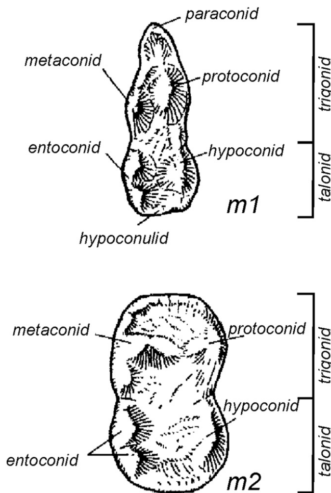
Fig. 6. The nomenclature of the elements of lower dentition of cave bear ( Ursus spelaeus ) used in this paper (after Baryshnikov, 2007).
