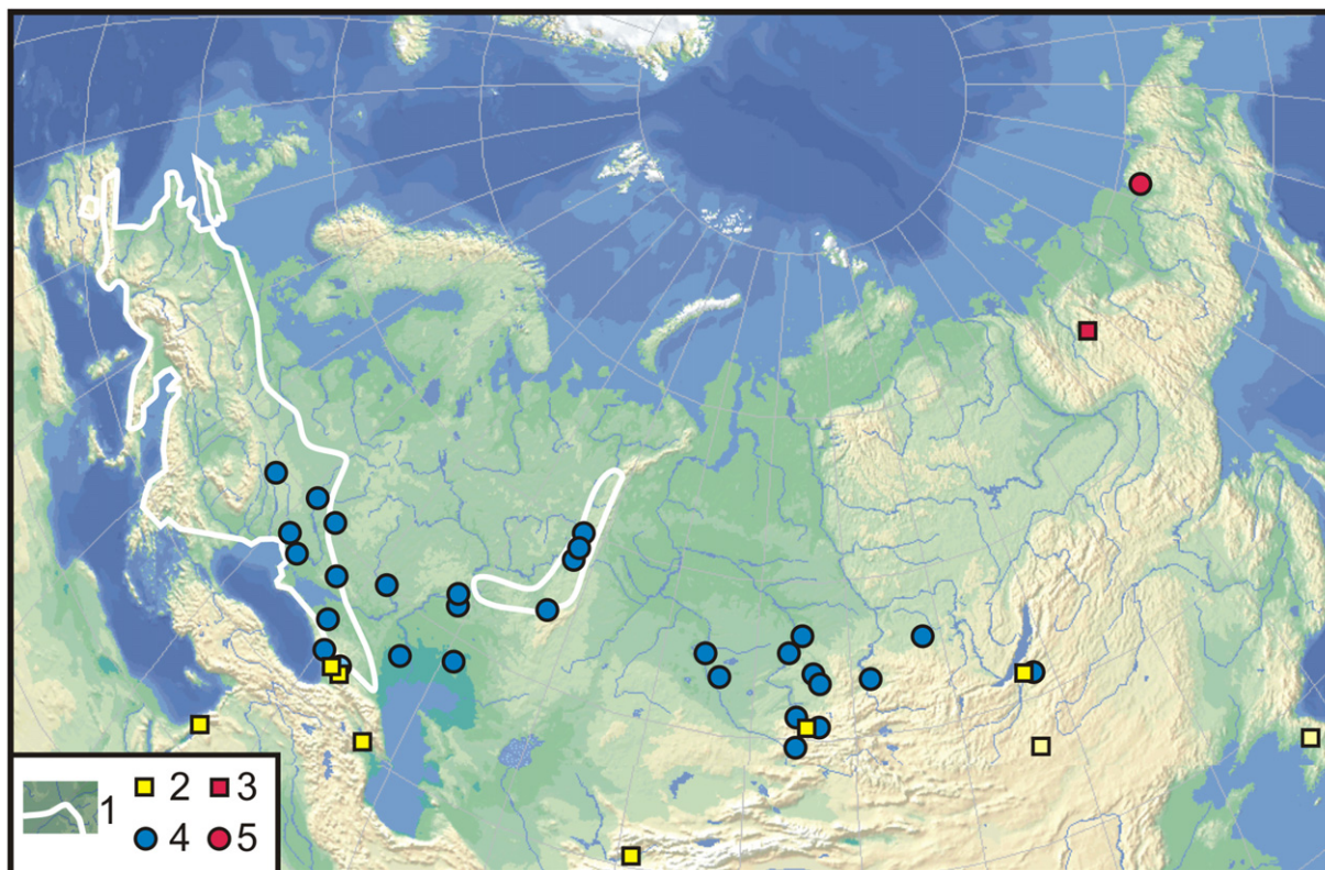
Fig. 1. Map with currently accepted distributions of various cave bears and the position of new findings (Adycha and Cherskiy). 1 – the European range of Ursus spelaeus and Ursus deningeri (after Kahlke, 1994); 2 – Asian findings of U. deningeri (after Baryshnikov and Kalmykov, 2005 and Baryshnikov, 2007); 3 – new find of U. cf. deningeri in northeastern Siberia (Adycha); 4 – findings of U. savini rossicus and U. savini uralensis (after Vereshchagin and Baryshnikov, 2000; Baryshnikov, 2007); 5 – Lower Kolyma River, Cherskiy locality of Ursus savini nordostensis subsp. nov.
